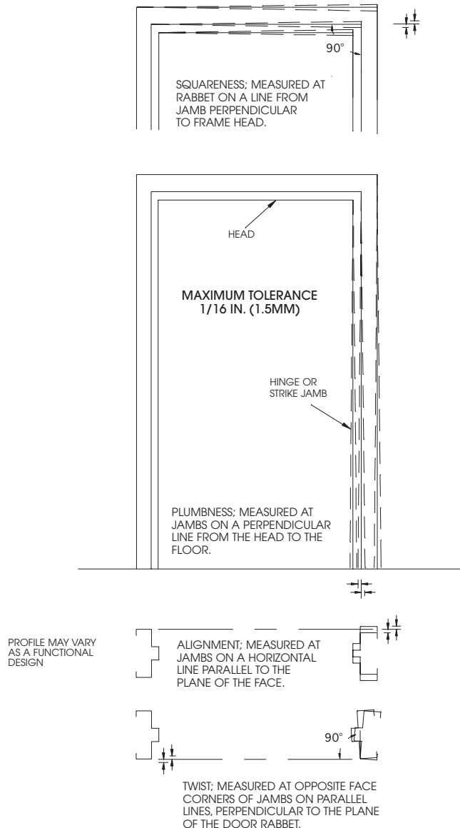
FIGURE 6 Installation Tolerances
