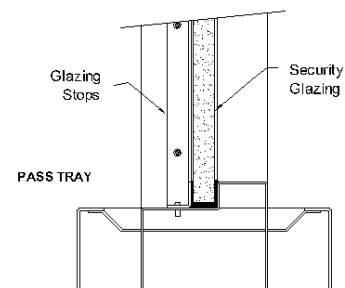
FIGURE 3 Typical Control Room Details
