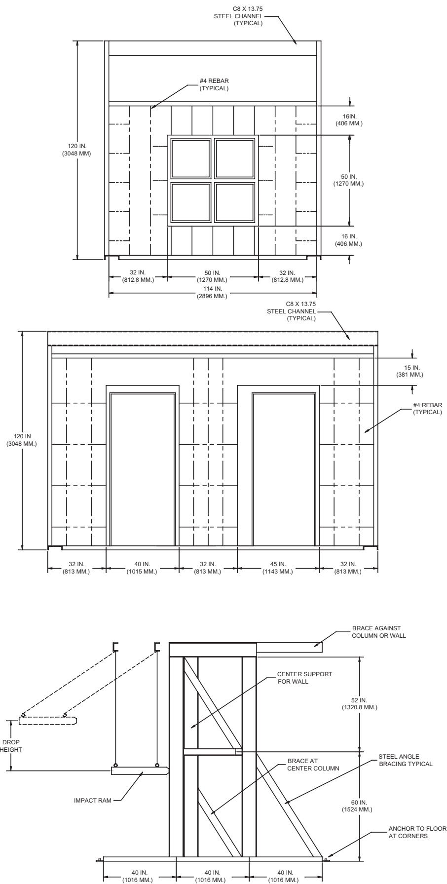
FIGURE 1 Test Wall
