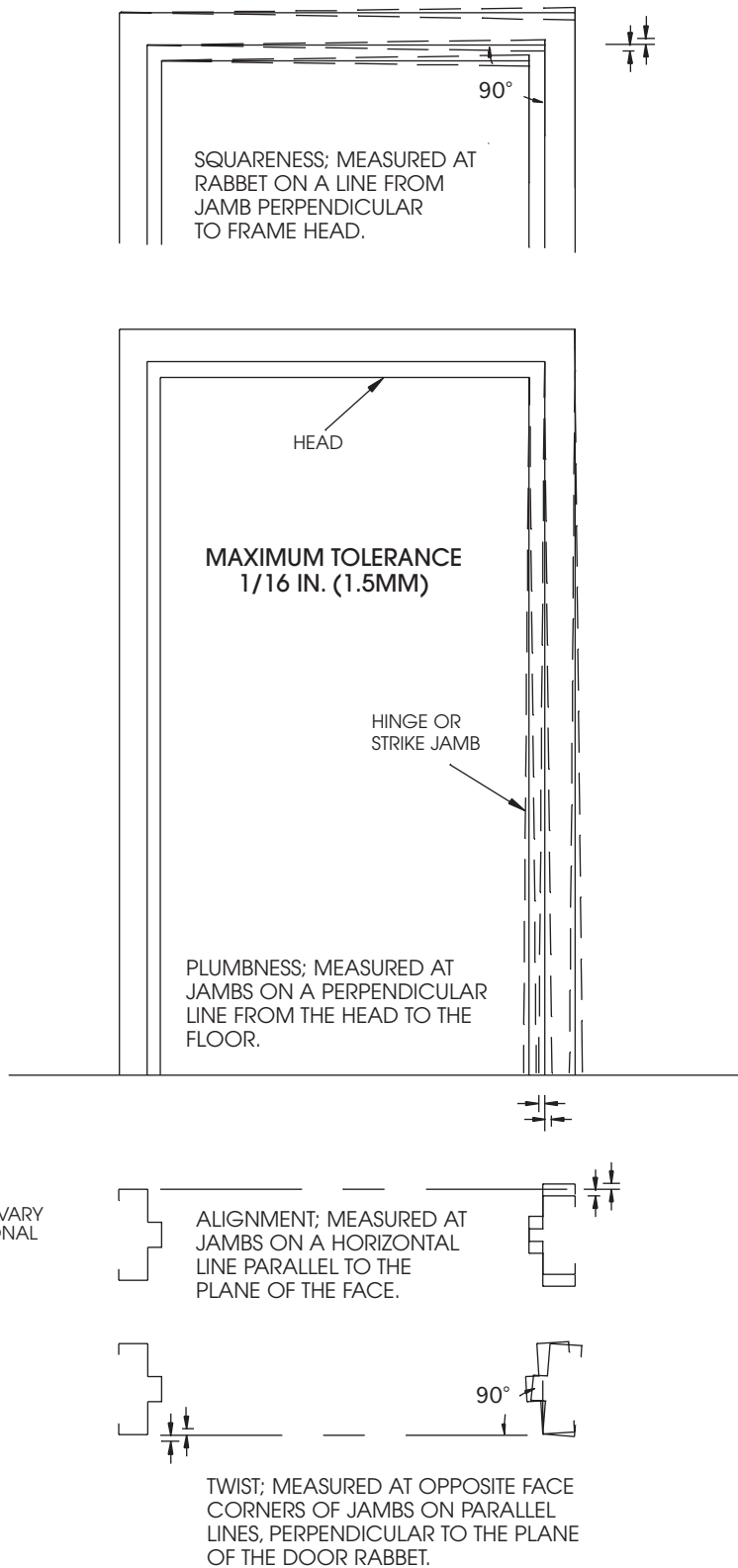
FIGURE 12 Installation Tolerances
