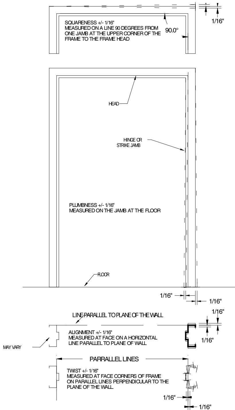
FIGURE 3 INSTALLATION TOLERANCES
