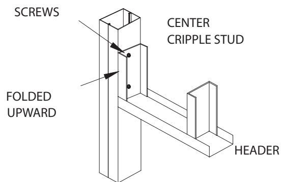
FIGURE 16A RECOMMENDED
