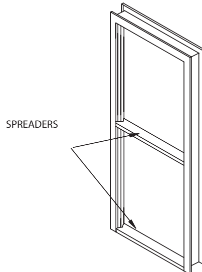
FIGURE 6 SPREADER LOCATION
