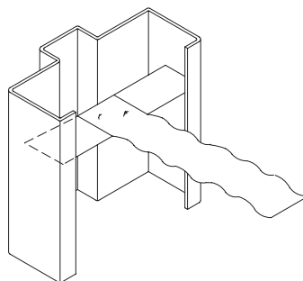
FIGURE 14C T-STRAP ANCHOR
