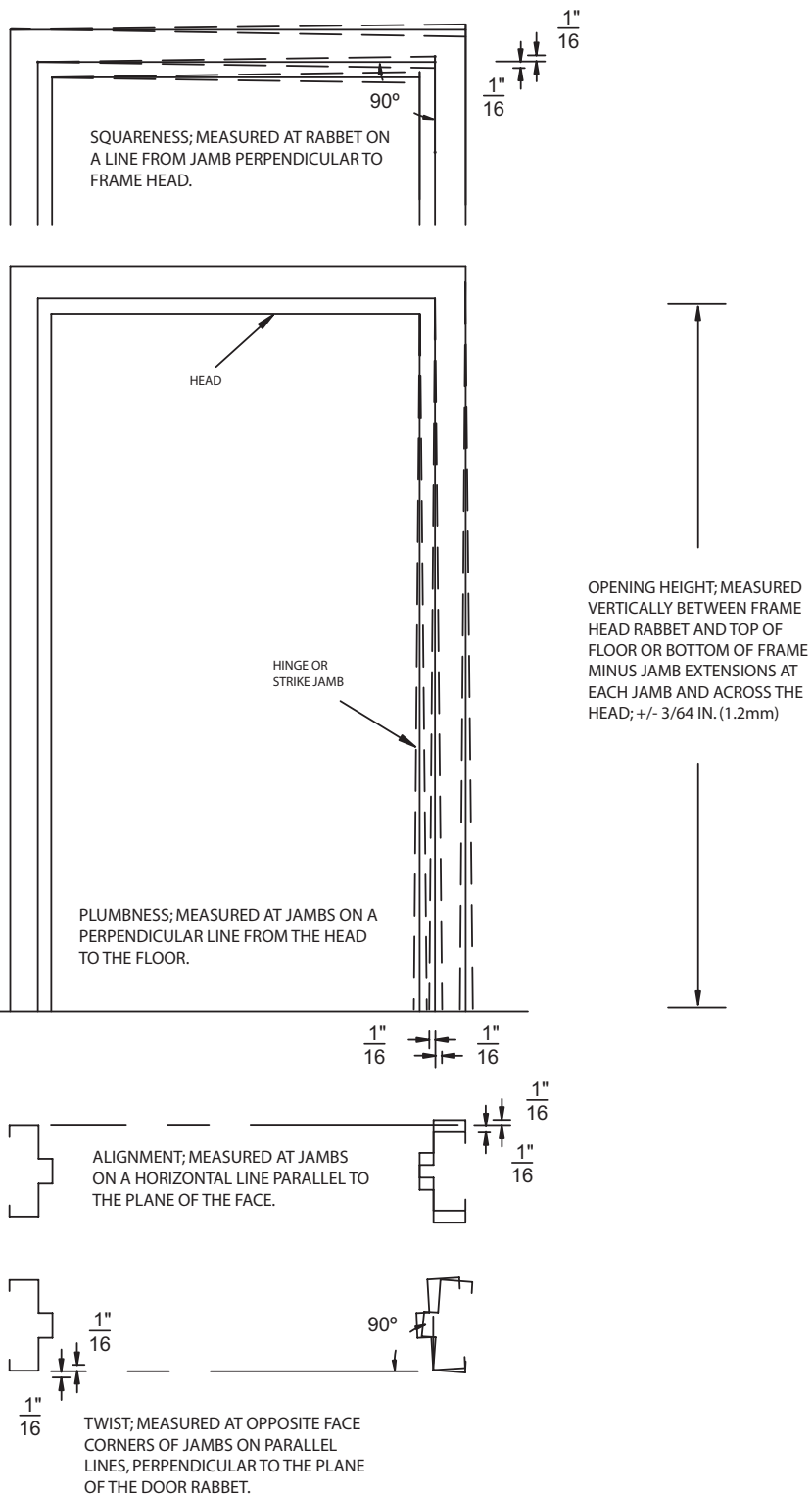
FIGURE 3 FRAME INSTALLATION TOLERANCES
