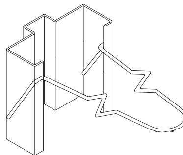
FIGURE 14D WIRE LOOP ANCHOR
