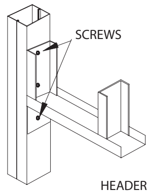
FIGURE 16B ACCEPTABLE
