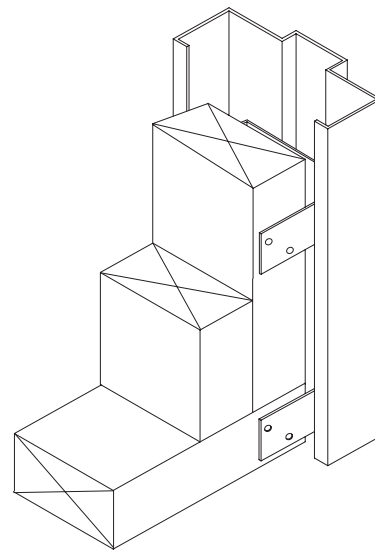
FIGURE 17E WOOD STUD WALL WITH ANCHORS
