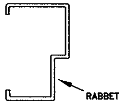
Single Rabbet
