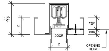
1 HEAD ASSEMBLY
